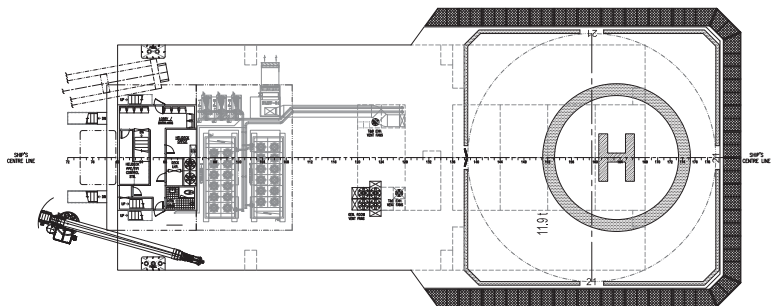
Helideck
