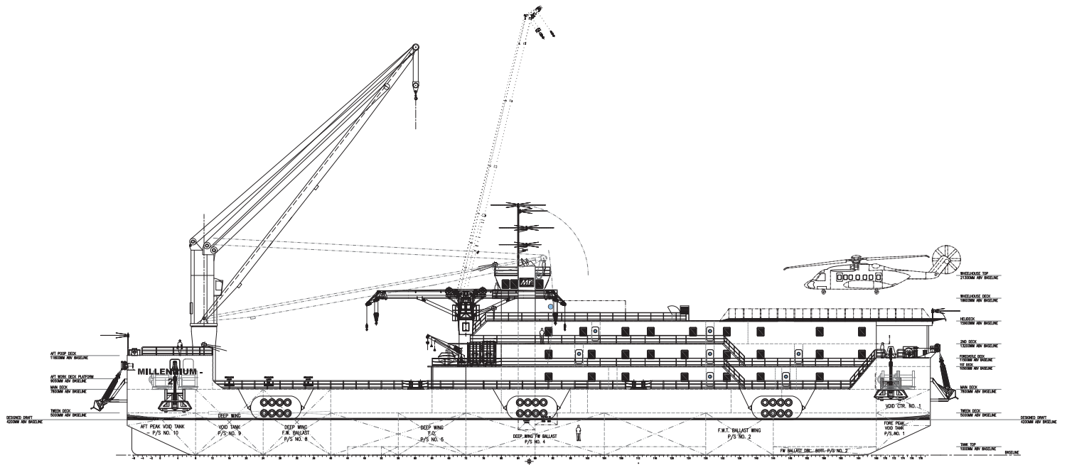
Outboard profile
