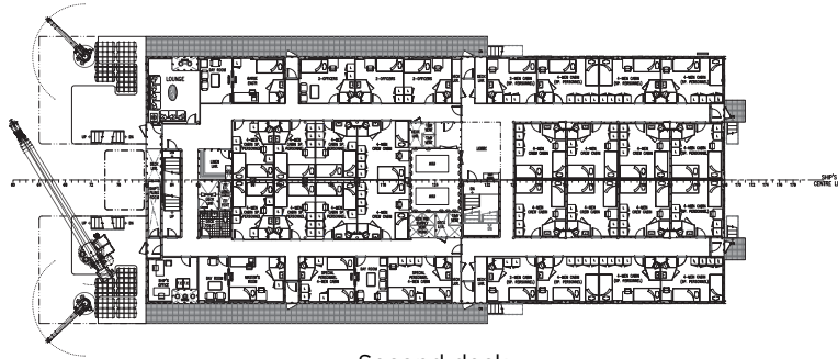
Second deck
