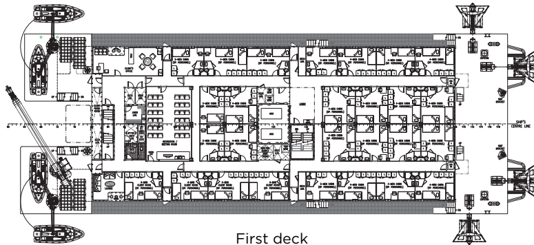
First deck
