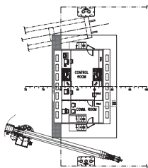
Wheelhouse deck
