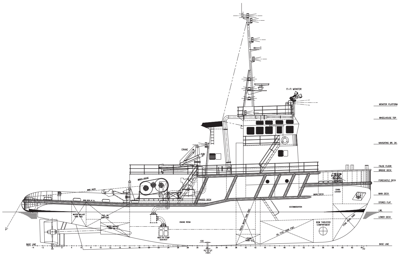
Outboard profile
