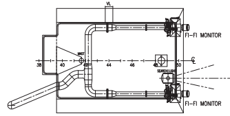
Monitor platform
