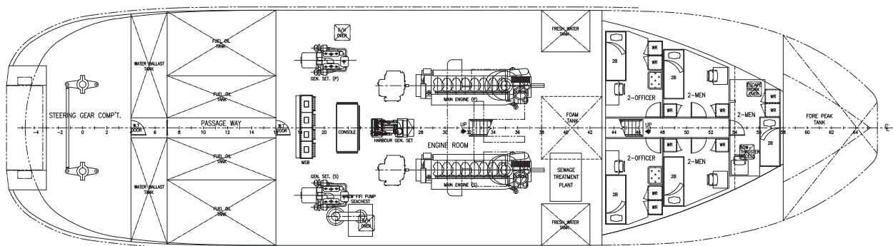
Below main deck plan
