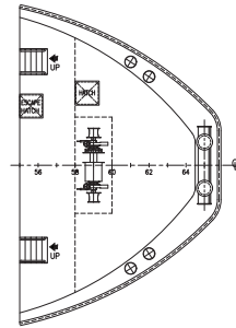
Forecastle deck
