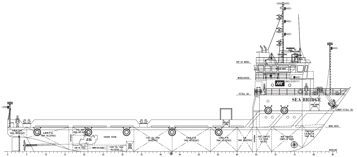
OUTBOARD PROFILE
