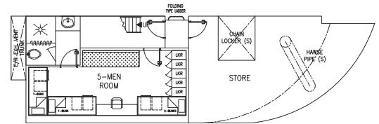
LOWER FORECASTLE DECK
