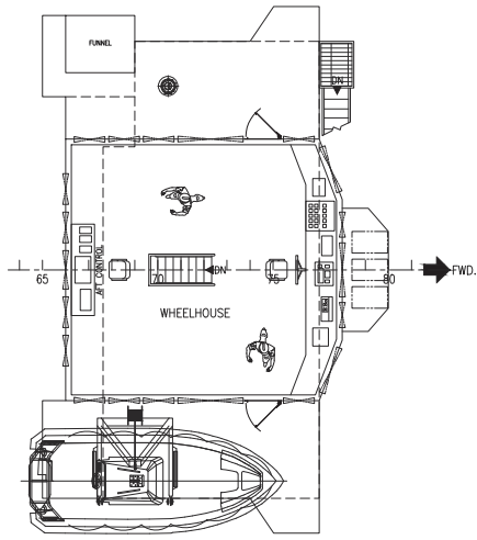
WHEELHOUSE DECK
