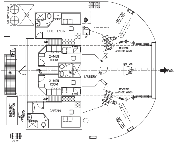
FORECASTLE DECK
