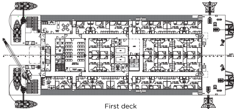
First deck
