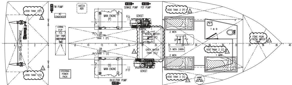
Below main deck plan
