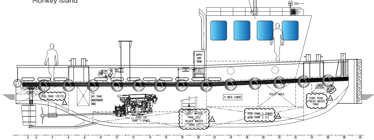
Outboard profile
