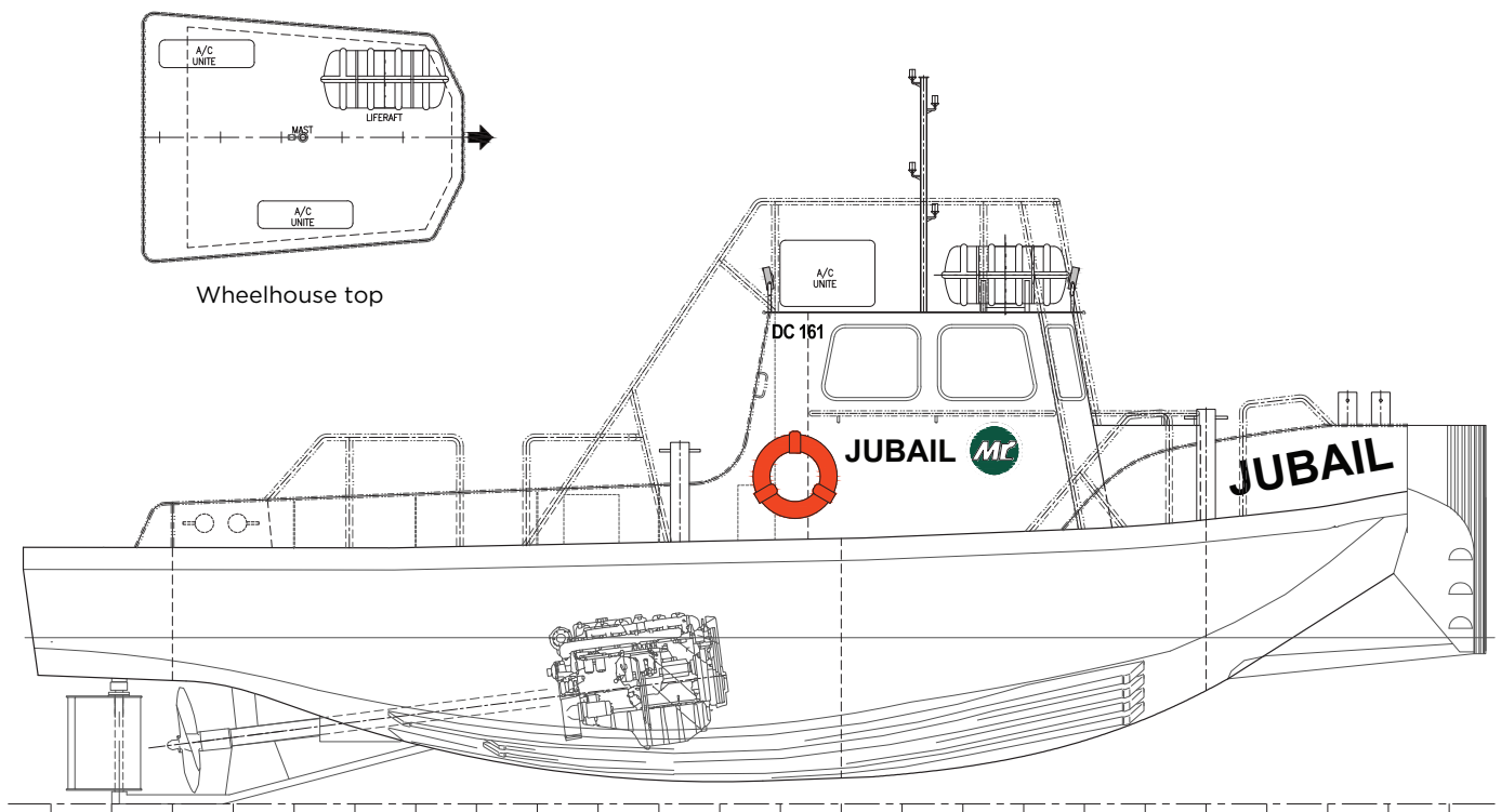
Outboard profile
