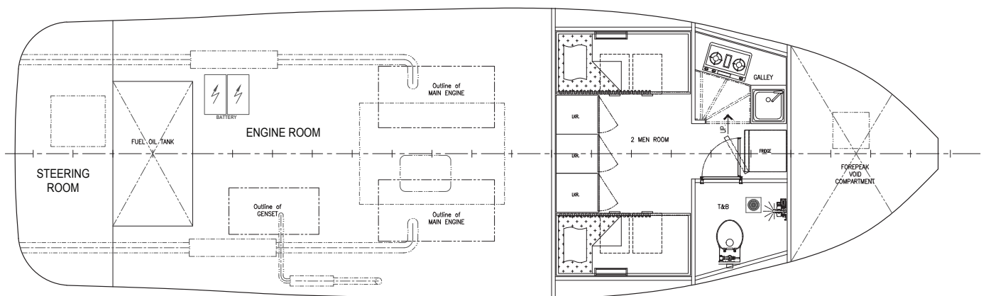
Below main deck plan
